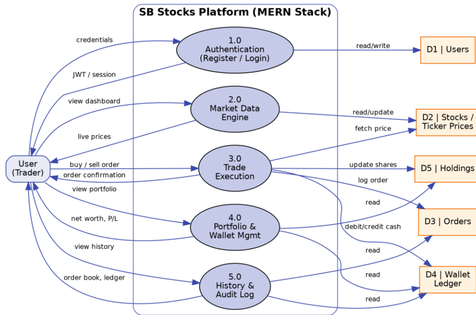
Figure 1: Data Flow Diagram (Level 1) – SB Stocks Trading Platform
